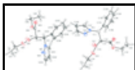
Fig. 1. Molecular structure of the title compound with the atom-labelling scheme. Displacement ellipsoids are drawn at the 50% probability level.
