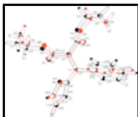
Fig. 2. View showing the fitting between the molecule 1 and the inverted molecule 2 from the asymmetric unit [PLATON (Spek, 2009)].
